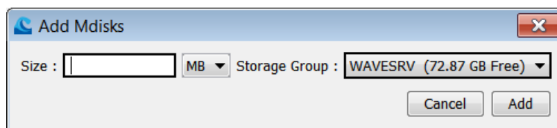
Figure 72. Add Mdisks
