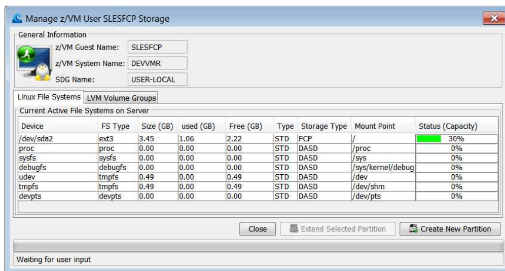
Figure 89. Manage Storage
