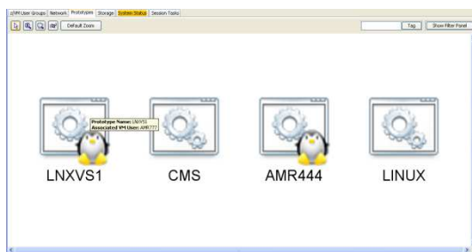
Figure 47. Prototype viewer
