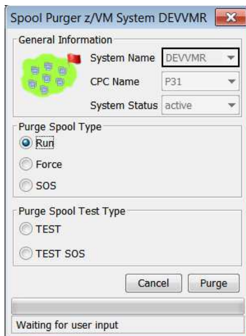
Figure 69. Purge Spool
