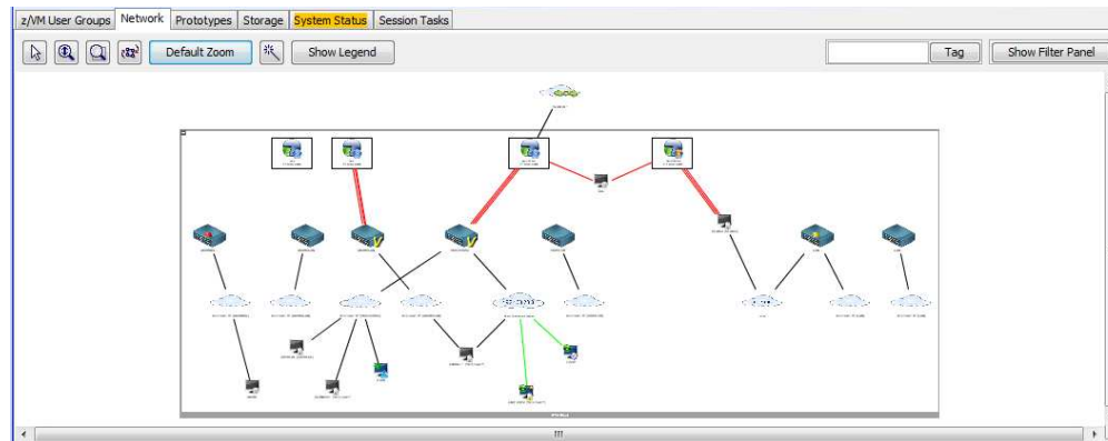
Figure 34. Network Viewer
