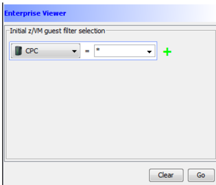
Figure 19. Enterprise viewer
