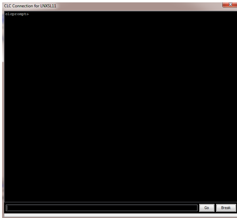
Figure 77. CLC editor
