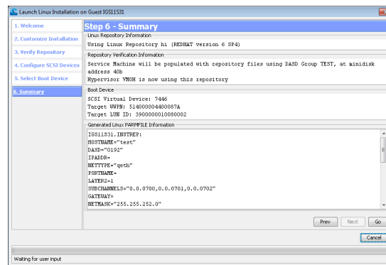
Figure 88. Step 6 - Summary
